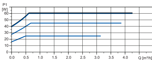
Constant curve
