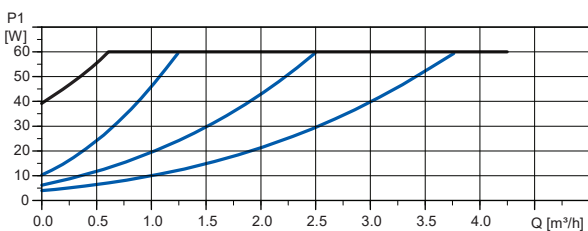
Proportional pressure
